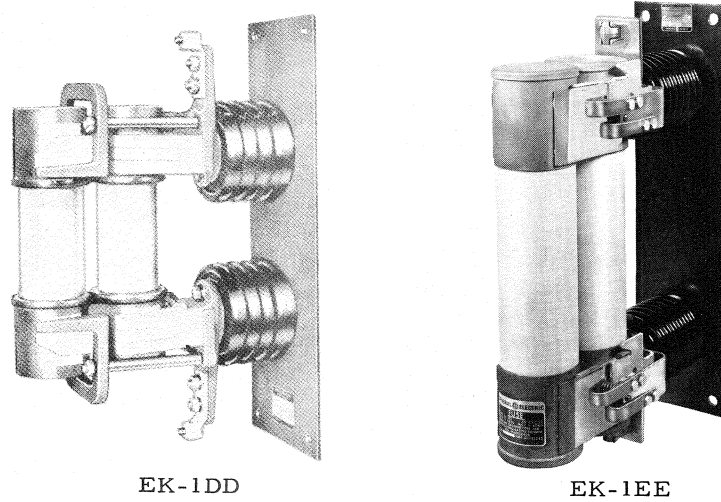
Fig. 1. Type EK-1 fuse supports (indoor) †
