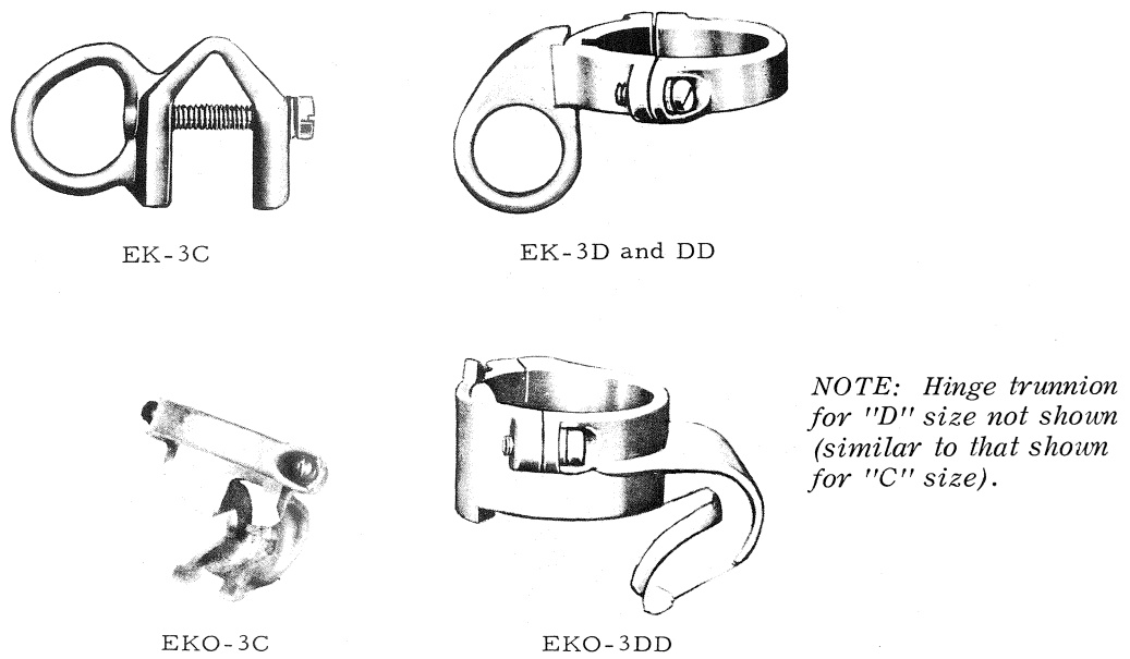
Fig. 8. Fuse fittings for Type EK-3 and EKO-3 fuse-disconnecting switches
