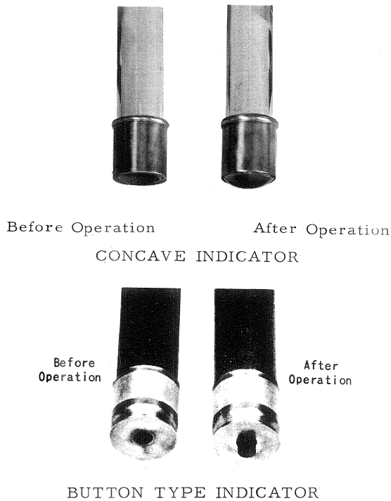
Fig. 9. Typical blown fuse indicators
