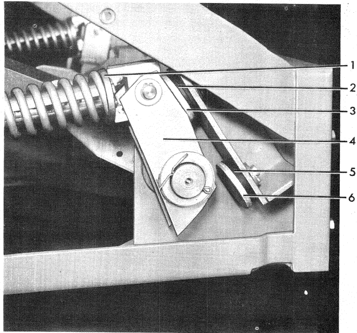
Fig. 5 Buffer Assembly
