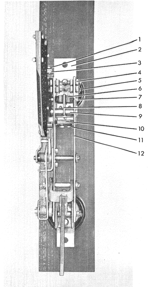
Fig. 8 Contact Arrangement
