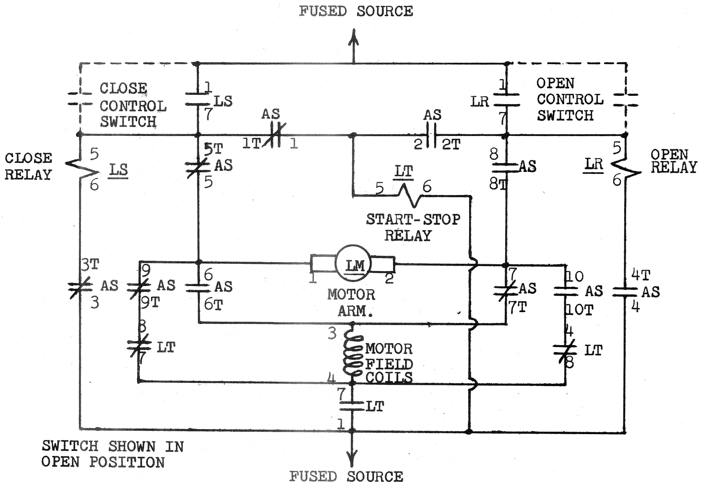
Fig. 12 SCHEMATIC WIRING DIAGRAM
