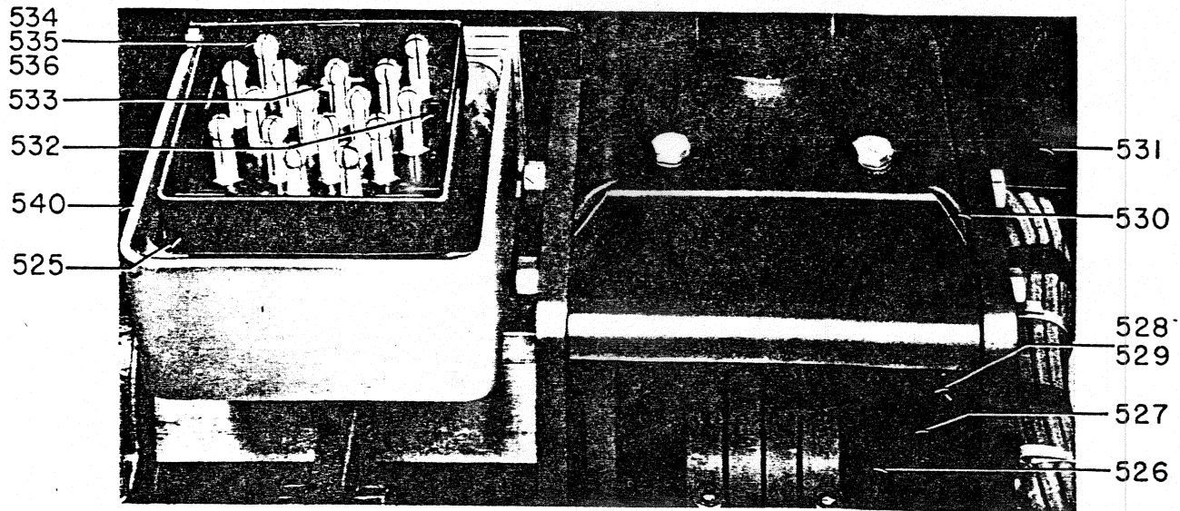
Fig. 12. Secondary disconnecting device; and mechanism parts
