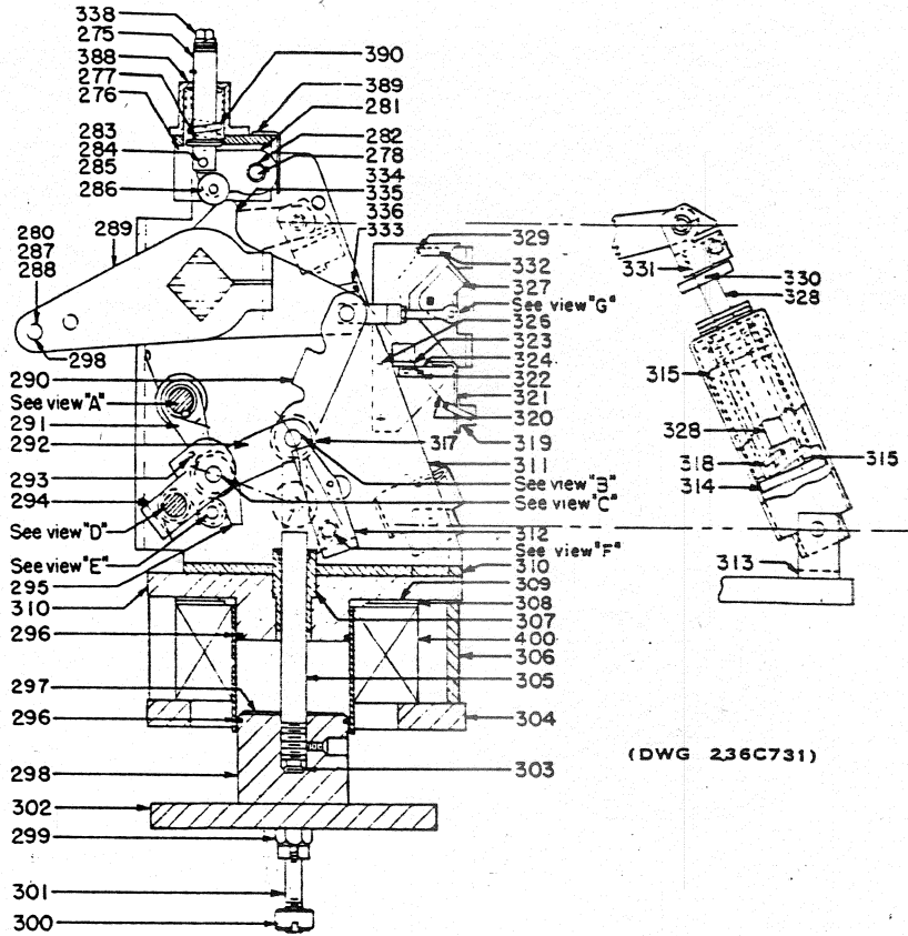
Fig. 8. Cross-section of mechanism for type AM-13.8-1 and -2 breakers
