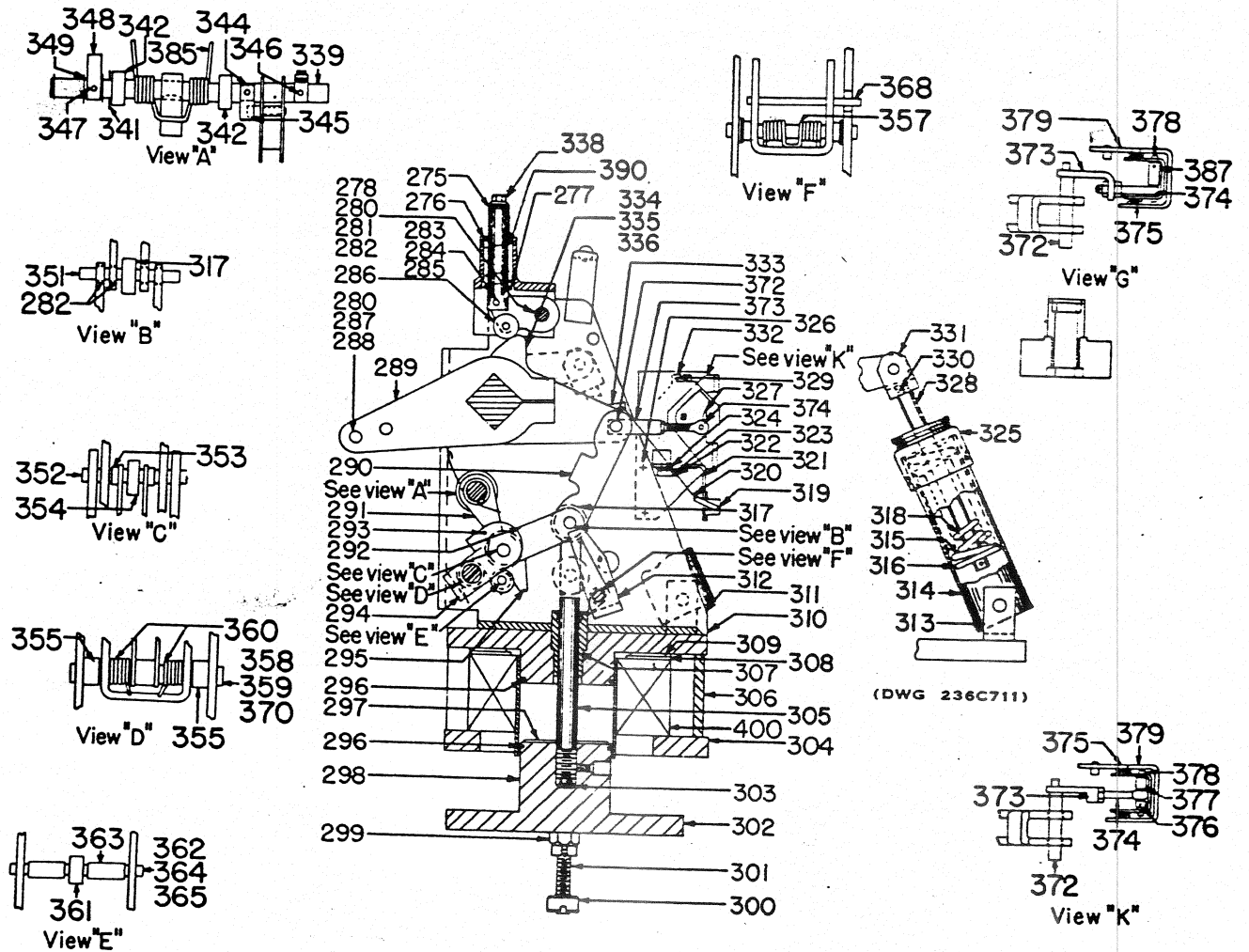
Fig. 7. Cross-section of mechanism for type AM-13.8-0 breaker
