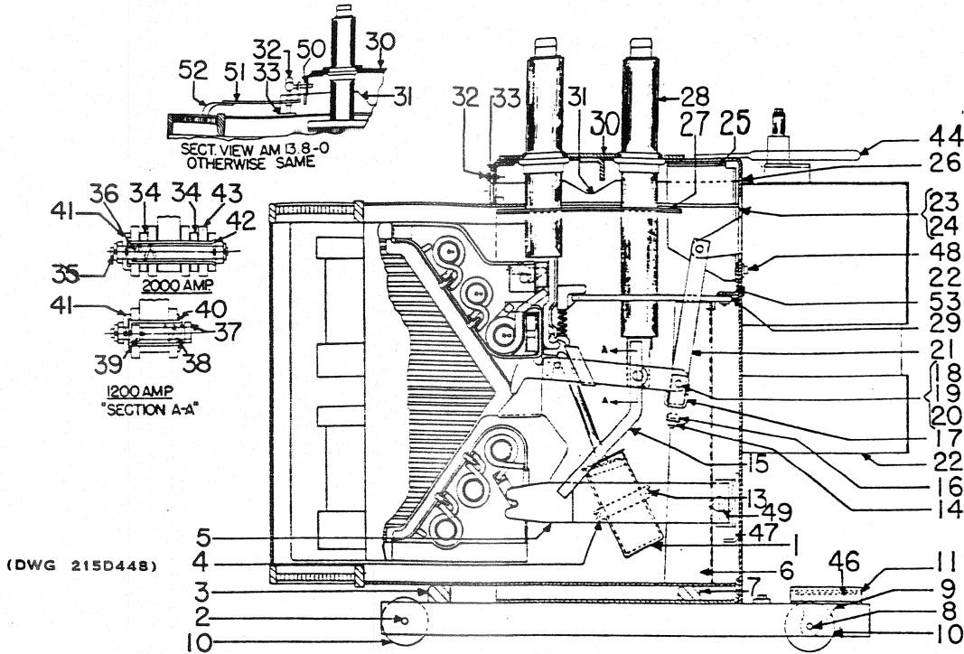
Fig. 2. Cross-section view of breaker PARTS REFERENCED IN FIG. 2
