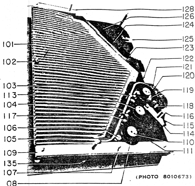
Fig. 3. Arc chute assembly with side cover removed
