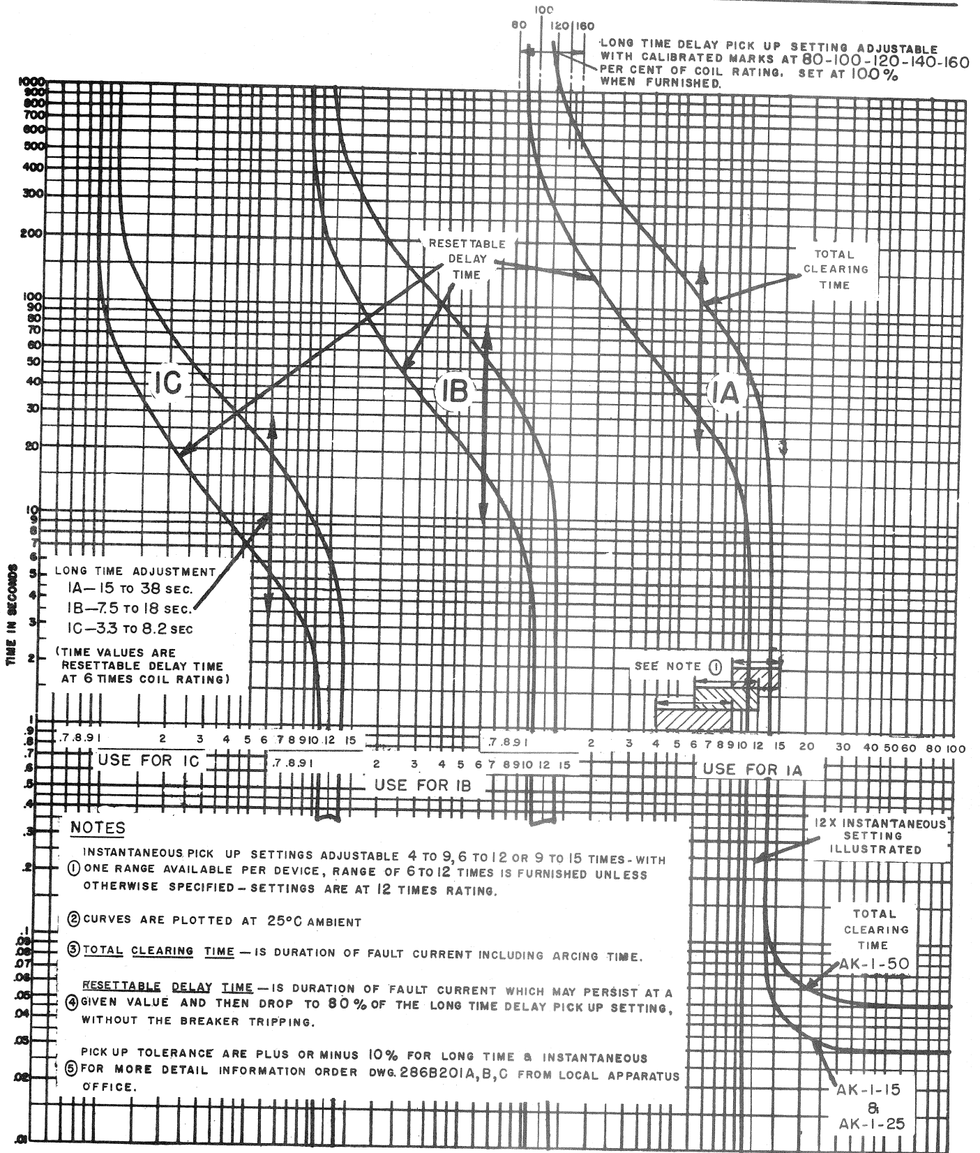
Figure 6. Time-Current Characteristic of the Type EC-2 Overcurrent Trip Device
