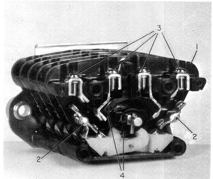
Fig. 2 Partially Dis-assembled SB-12 Auxiliary Switch
