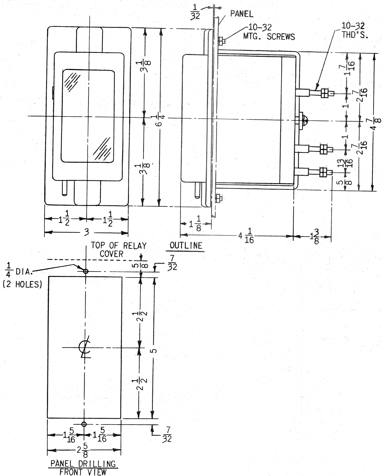
Fig.6 (0127A9555-1) Outline And Panel Drilling Dimensions For The Semi-Flush Mounted HAA15A Relay
