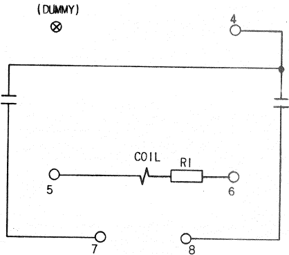
Fig.3 (0165A6061) Internal Connection Diagram Of The HAA15A Relay Showing Connections For Higher Amp Rating
