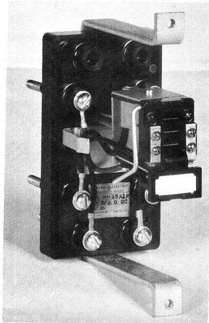
Fig. 1 (8030184) HAA15 Relay Removed From Case
